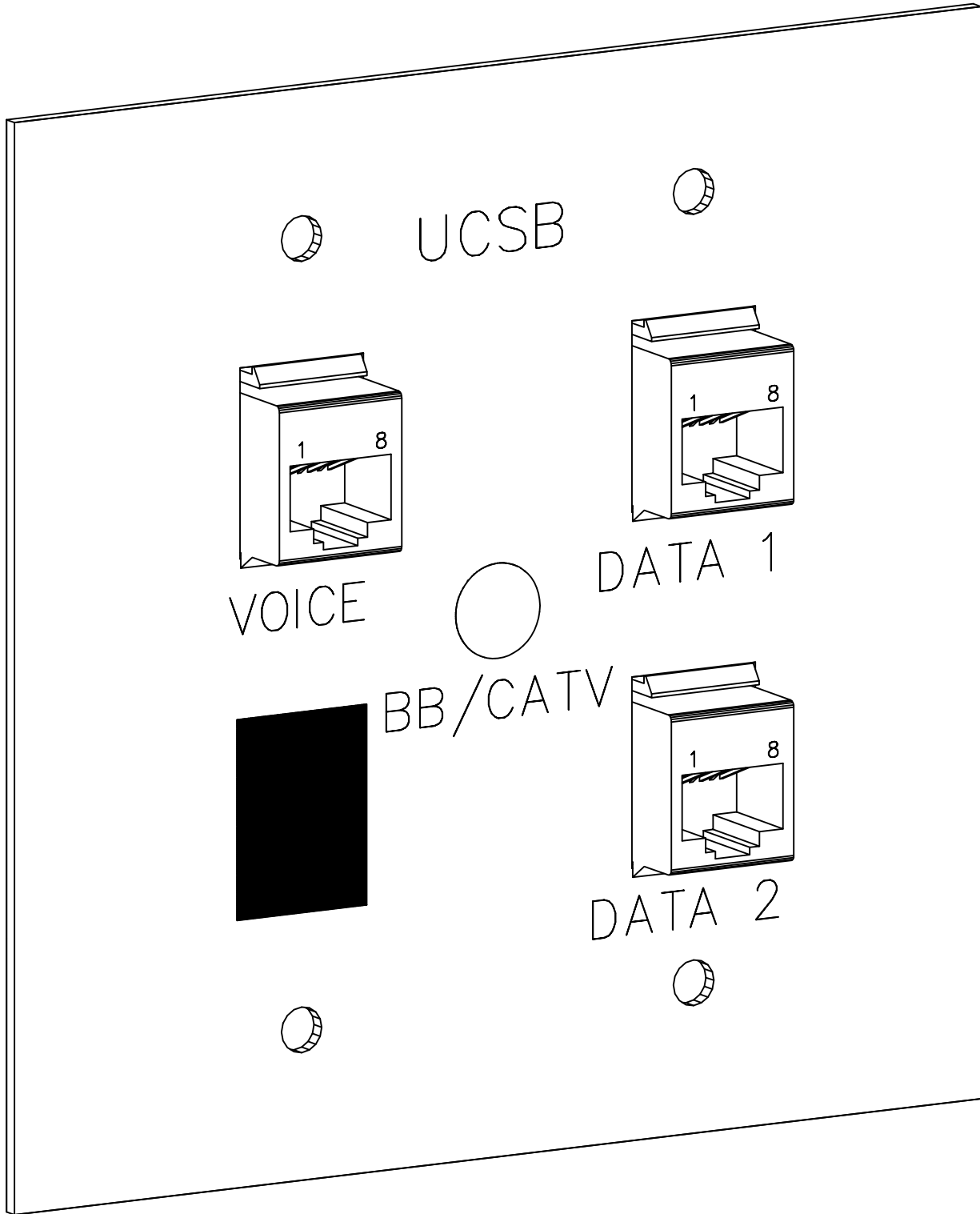
3D FRONT VIEW 4 X 4 WALLPLATE W/ 3 EIA/TIA 568A RJ-45 JACKS.
